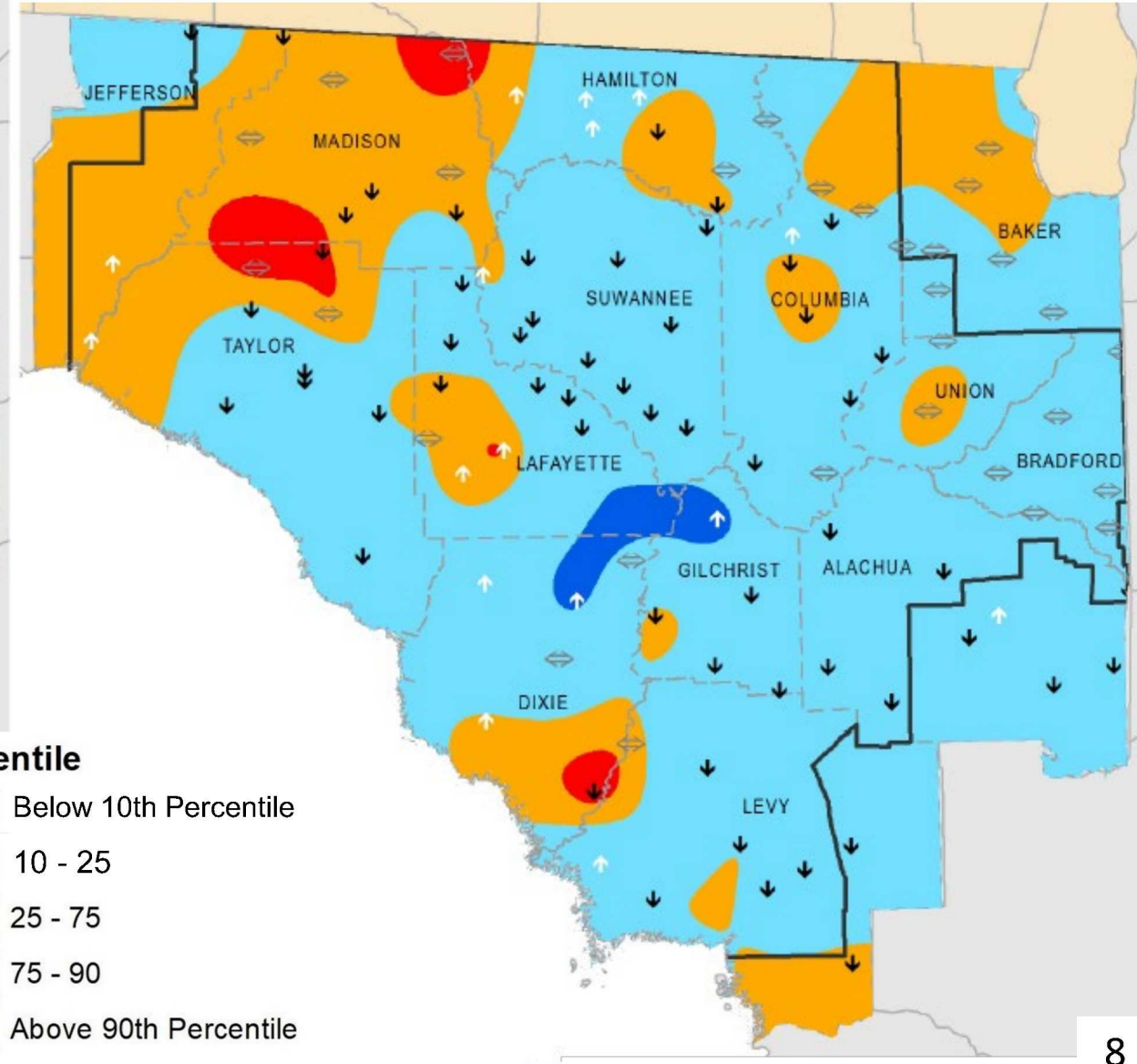
Upper Floridan Aquifer Levels End of December 2016
