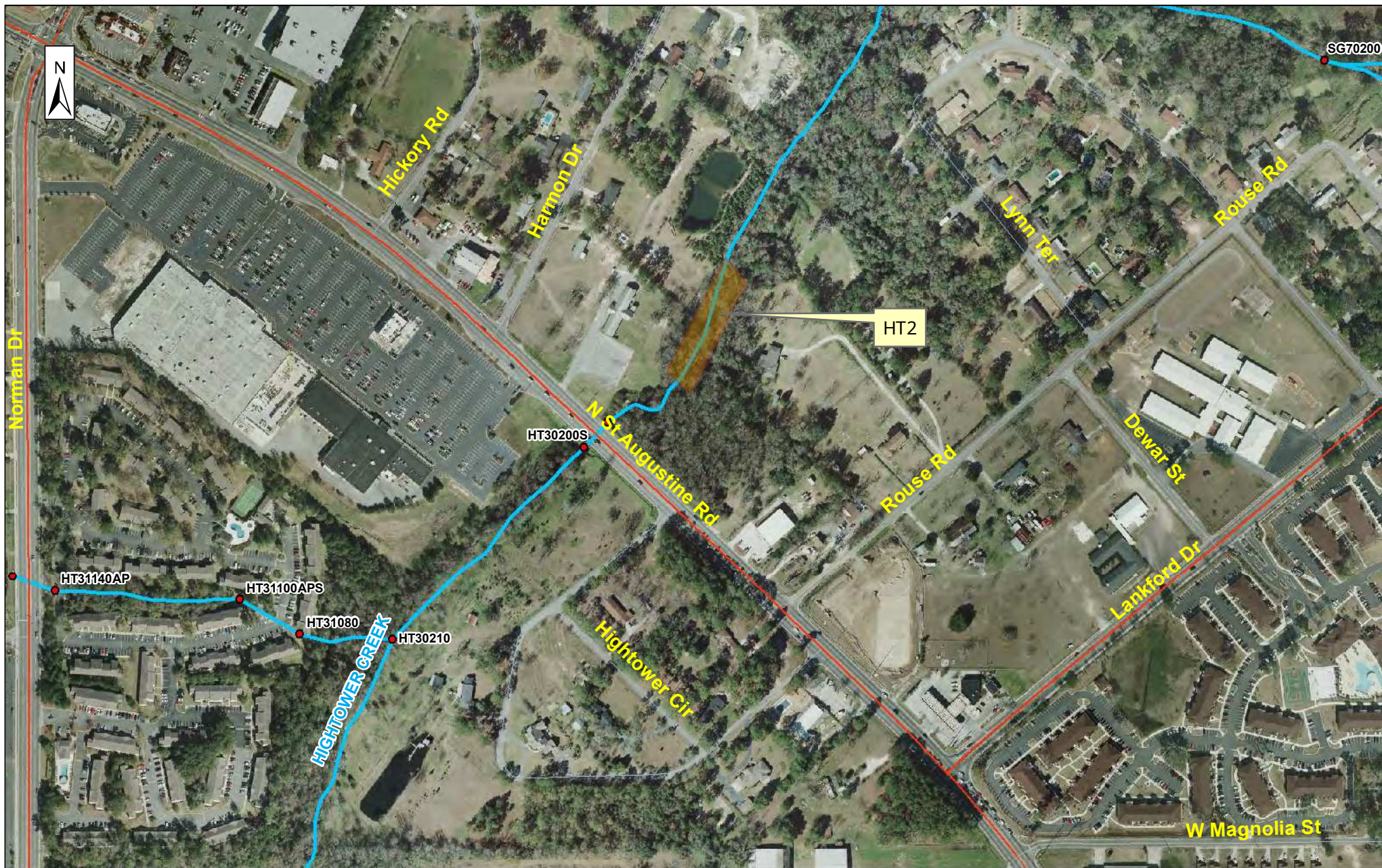
Figure 4.3.4 City of Valdosta, GA Hightower Creek Sub-basin Alternative HT2 Grade Control Structure Downstream of St. Augustine Rd
